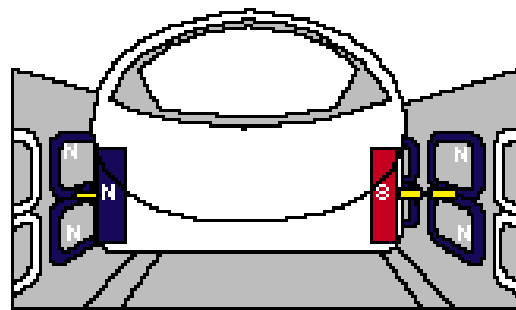
Principle of lateral guidance
