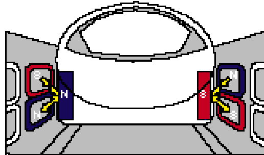
Principle of magnetic levitation
